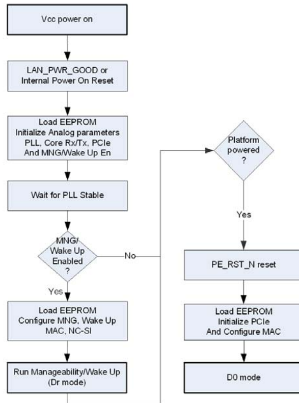
Figure 3-11. 82598 Power-Up Sequence
